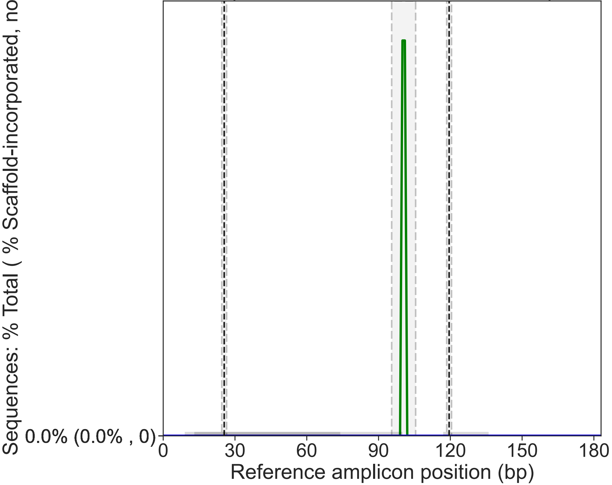
Mutation position distribution: Scaffold-incorporated
