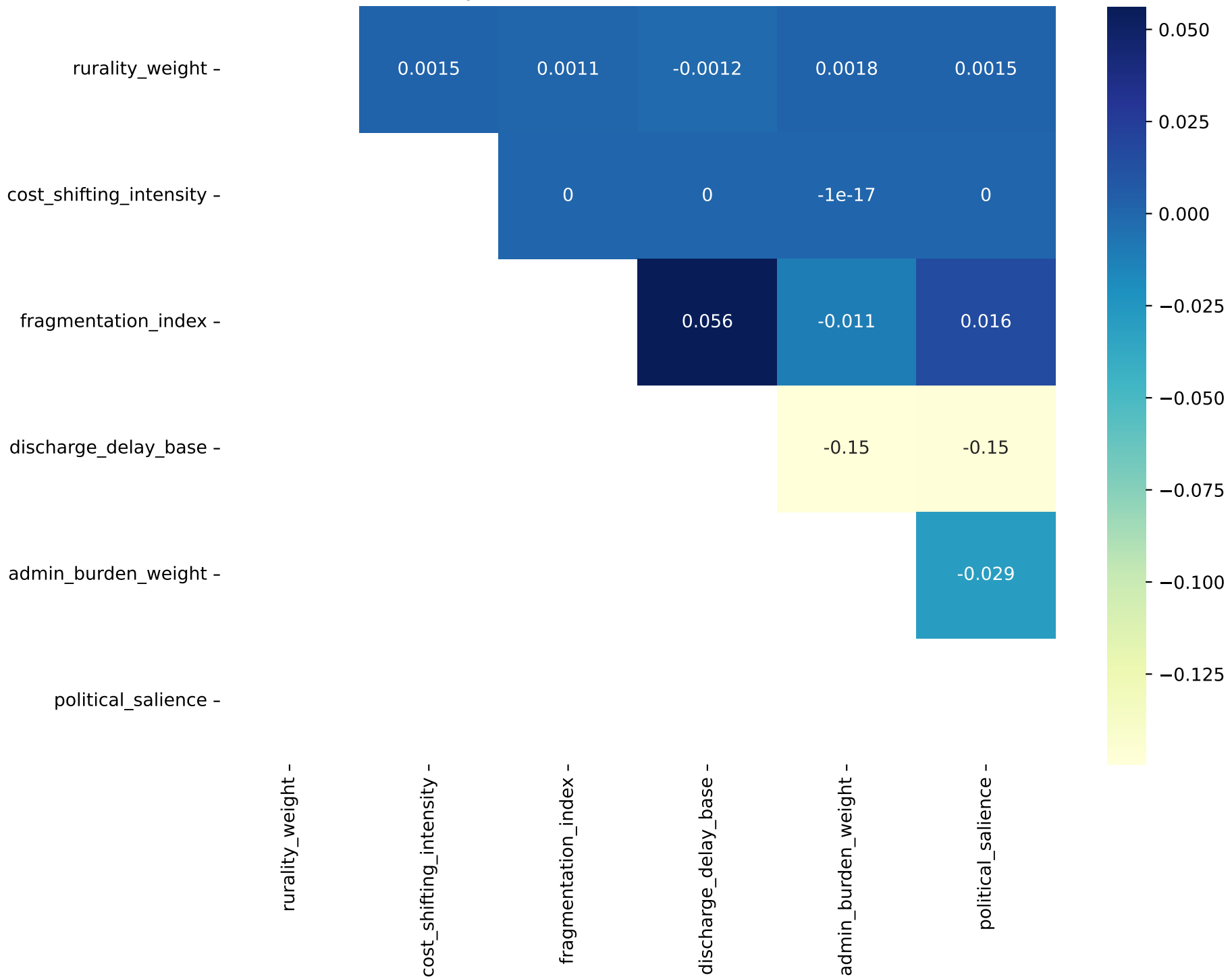
Sobol Analysis: Second-order Interaction Indices (S2)
