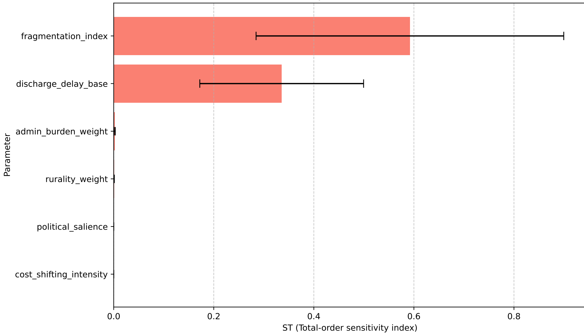
Sobol Analysis: Total-order Effects
