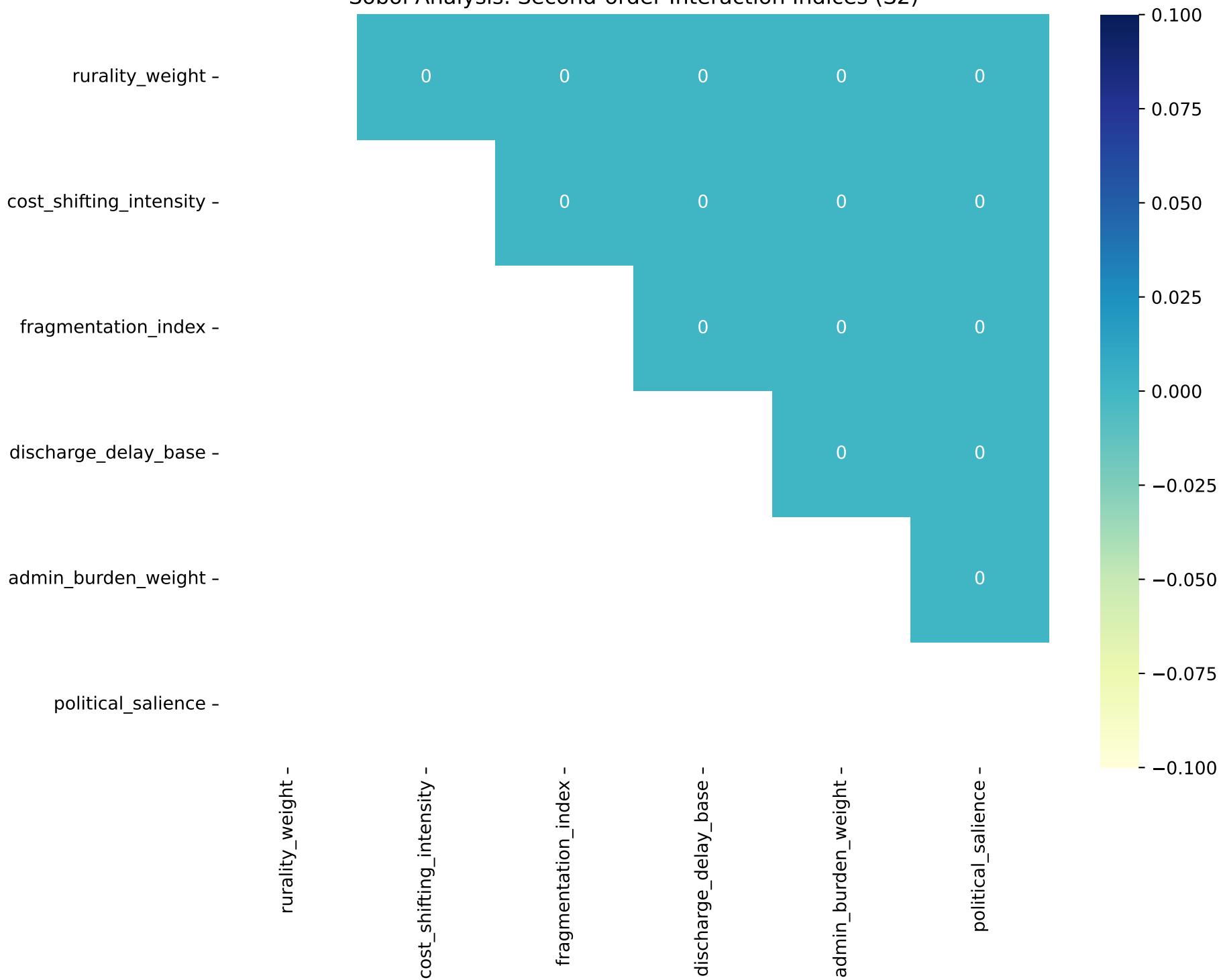
Sobol Analysis: Second-order Interaction Indices (S2)
