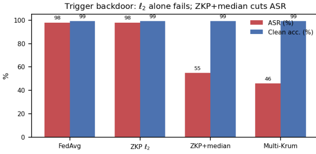
Fig. 3. Backdoor ASR vs. clean accuracy under FedAvg, l_2 -ZKP, ZKP+median, and Multi-Krum.
