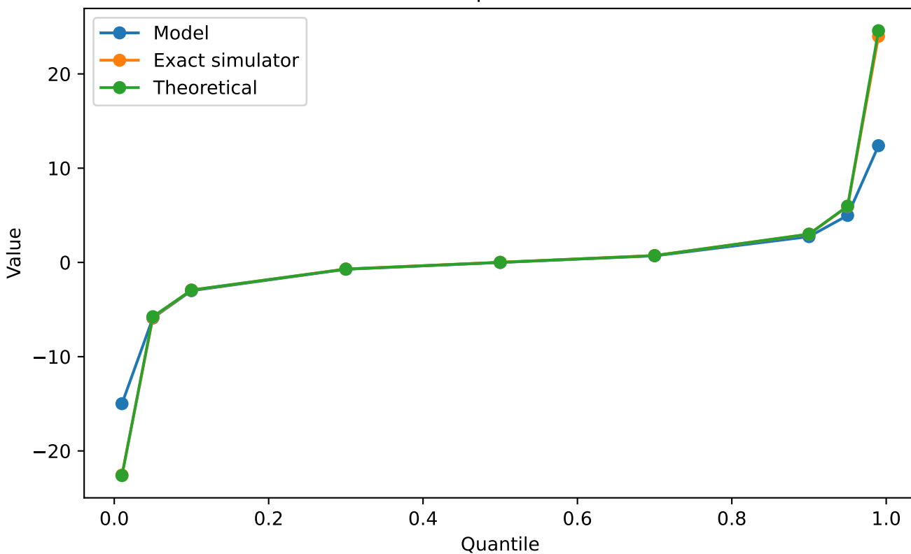
Component 5
