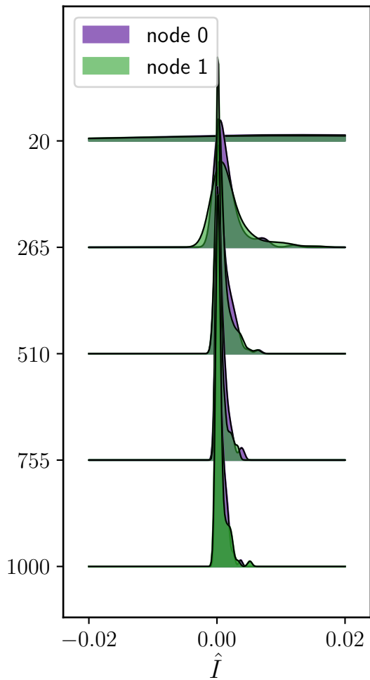
Gaussian
