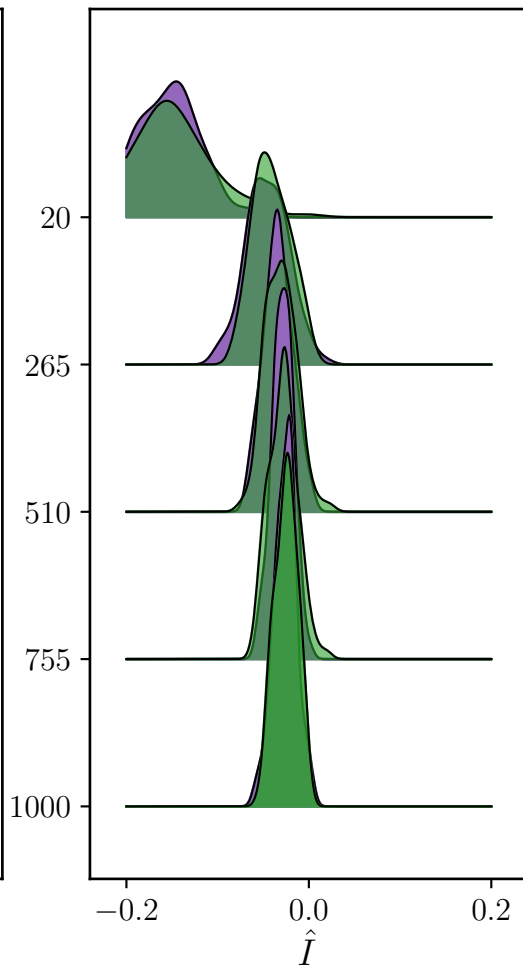
KNN cdtree
