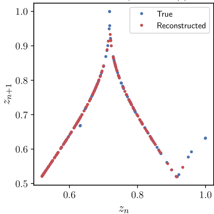
Successive maxima map of the z(t) variable
