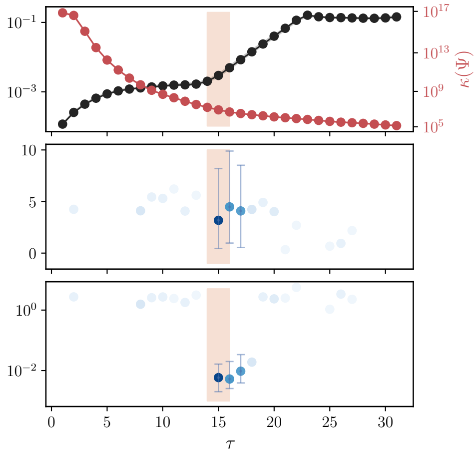
RK45 method
