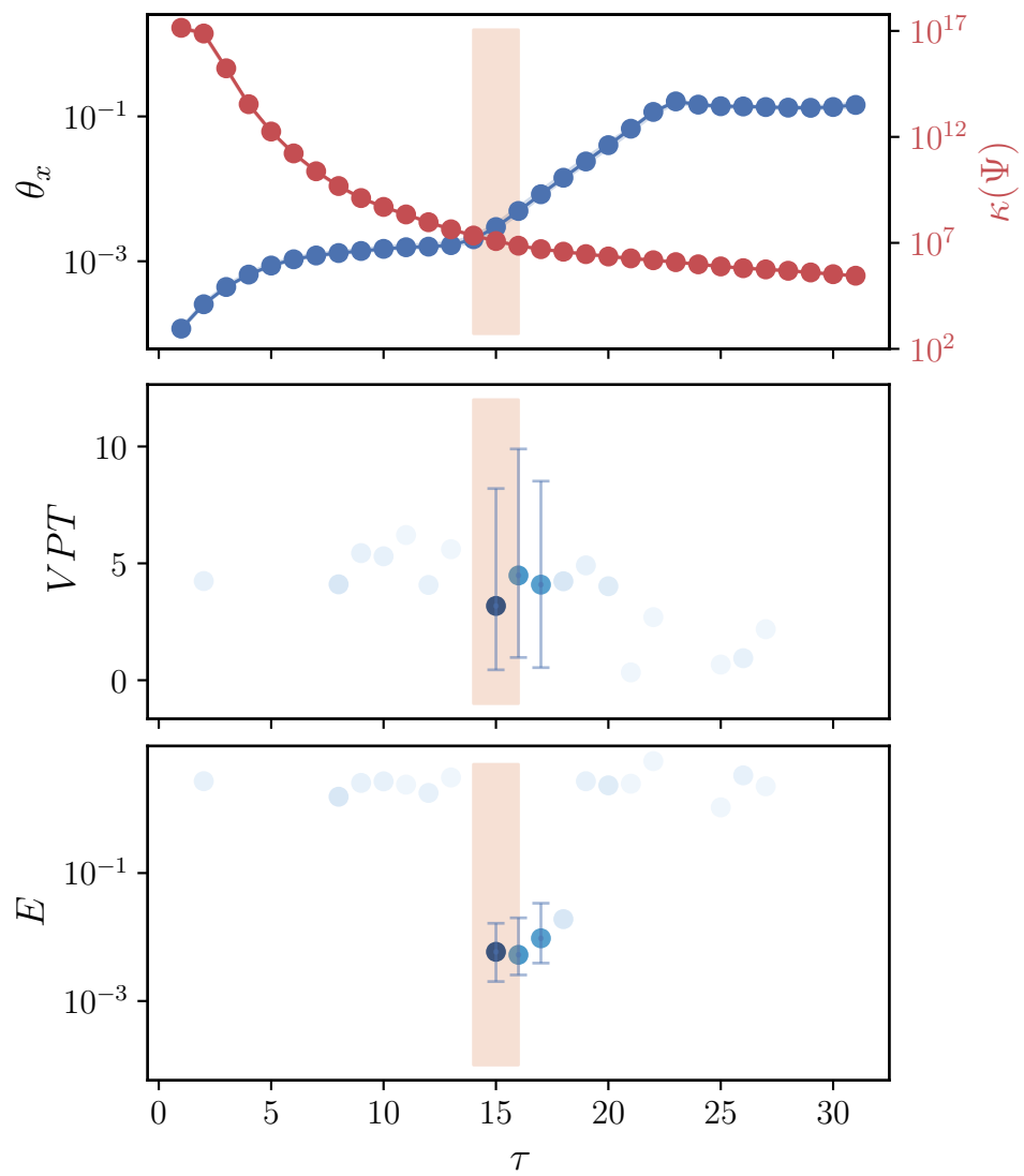
RK45 method
