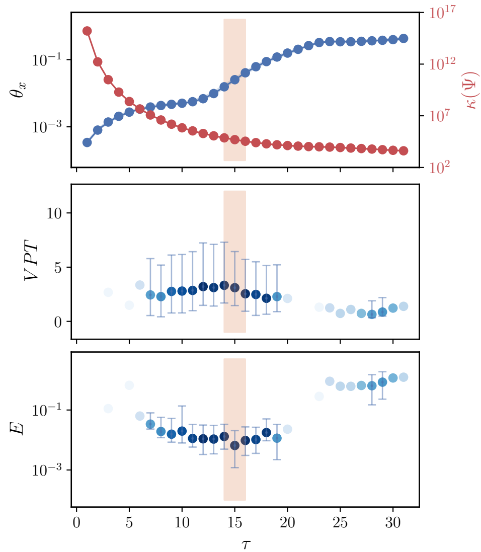
explicit Euler method
