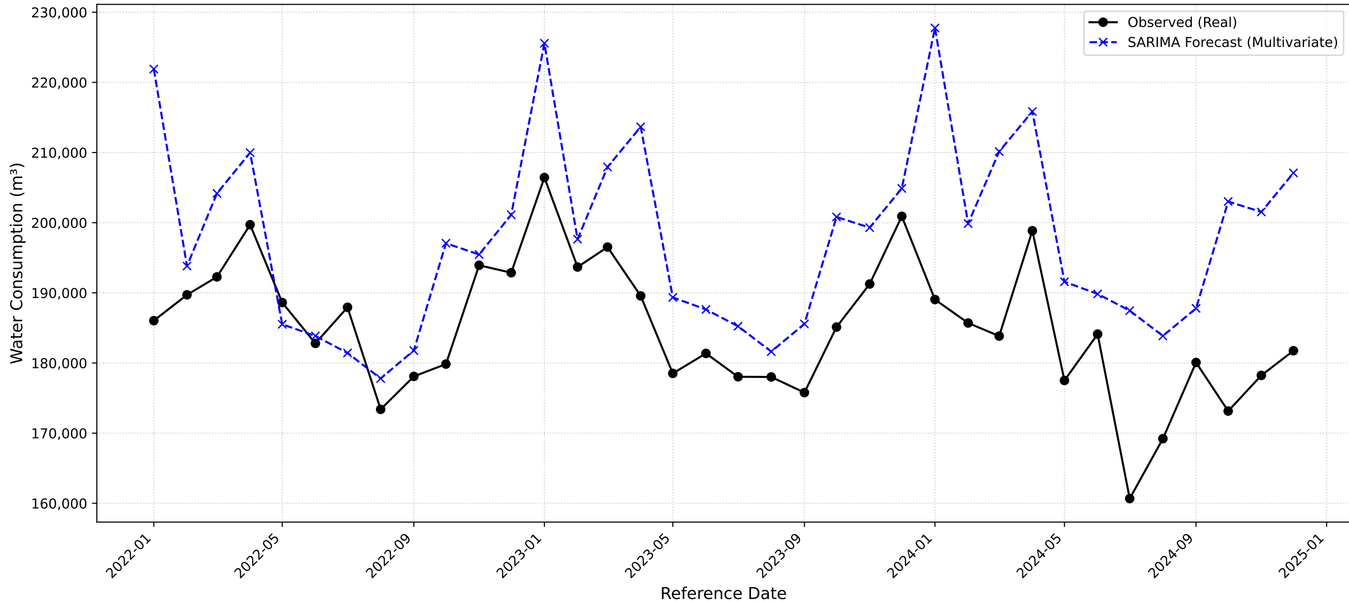
Consumption Forecasting Validation: SARIMA with Exogenous Variables (Features: Consumption + Population Growth + Income Growth | MAPE: 0.07%)
