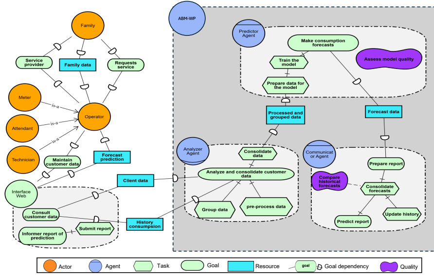
Figure 2: Architecture of the ABM-WP framework, encompassing the interaction between actors, tasks, and agents.
