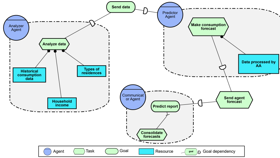
Figure 1: Tropos final requirements model with the AA, PA, and CA, using the piStar tool. Source: Elaborated by the author.
