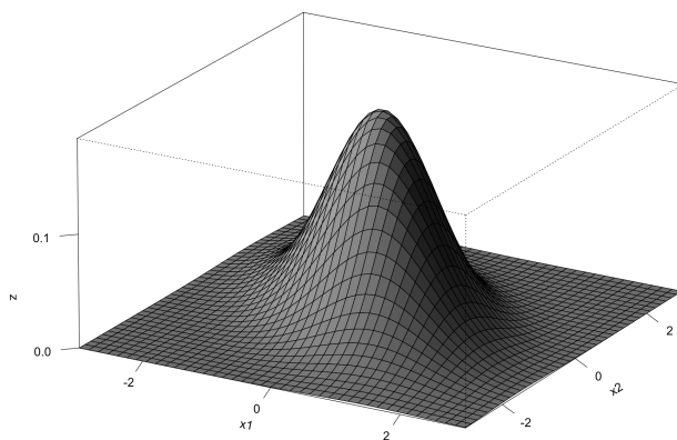
Figure 5.1: Bivariate Normal Distribution
