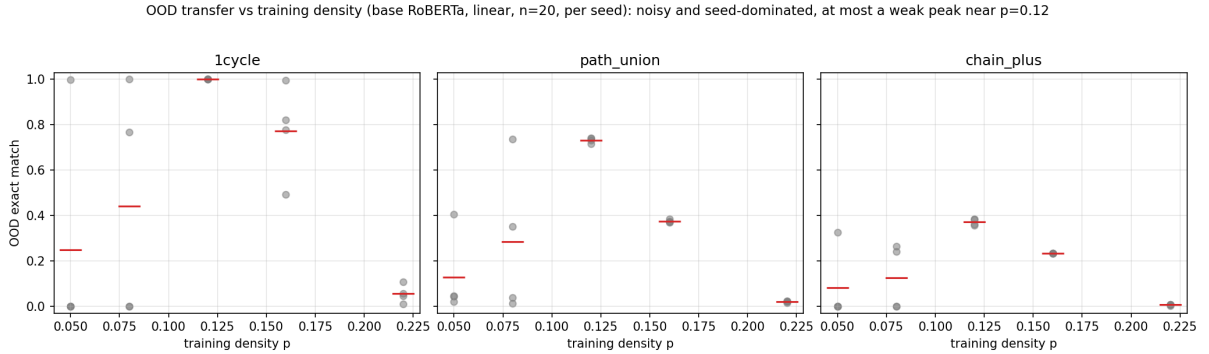
Figure 7: Model : the base connectivity transformer (RoBERTa-faithful trunk, linear read-out, L = 2 , single head, d_{\text{model}} = 512 ), ER (20, p )-trained, four seeds per density; eval-only . Test set : long structured families held out of the ER stream (1cycle, path-union, chain-plus), \geq 400 graphs each. Metric : OOD exact match vs training density p (grey dots = each seed, red bar = mean). Transfer is noisy and seed-dominated at the sparse end, peaks at p = 0.12 (and is cleanest there — all four seeds agree), and collapses for p \geq 0.16 as the dense training graphs stop exposing the model to long distances.
