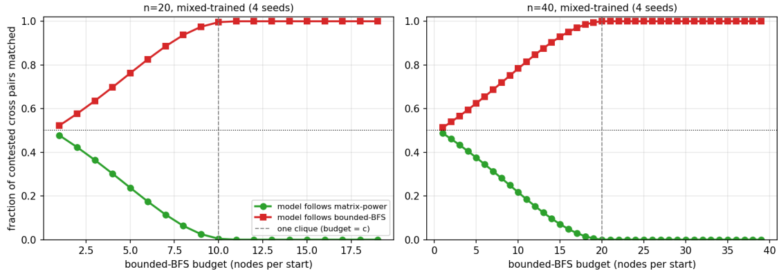
Figure 5: Model : the mixed -trained base connectivity transformer (RoBERTa trunk, linear read-out, L = 2 , single head, d_{\text{model}} = 512 , full-matrix \hat{R} ), eval-only, four seeds; n = 20 (left), n = 40 (right). Test set : bridged cliques at full clique size, 500 graphs. Metric : restricted to the cross pairs where the matrix-power oracle and the visit-bounded-BFS oracle disagree (the bridge pairs), the fraction the model matches to each oracle, as the BFS budget b varies. The model tracks the early-stopping BFS, not matrix powering: as b approaches one clique (dashed line) the model matches BFS on \rightarrow 1.0 of the contested pairs and matrix powering on \rightarrow 0 . This is the same fact as the cross collapse, read against the two reference algorithms.
