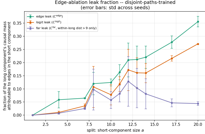
Figure 6: Table 3 as curves, mean over the four seeds, error bars = std across seeds.
