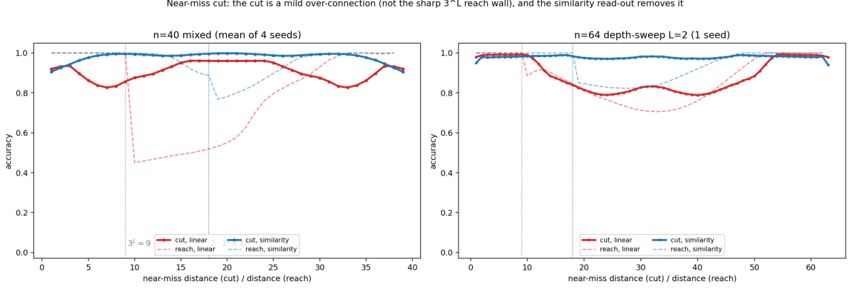
Figure 7: Near-miss cut test. Solid = cut accuracy vs near-miss distance; dashed = reach vs distance, same axis. Left: n = 40 mixed (mean of four seeds); right: n = 64 depth-sweep L = 2 (one seed). Reach drops sharply at capacity (9 linear, 18 similarity); the cut is a shallow, broad dip with no step there, and the similarity read-out flattens it to \approx 1.0 .
