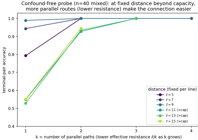
Figure 5: Table 19 for the mixed model (standard linear read-out, n = 40 ). Each line is a fixed distance \ell ; the beyond-capacity lines ( \ell = 11, 13, 15 ) climb steeply with k — at the same distance, more parallel routes (lower resistance) make the connection easy.
