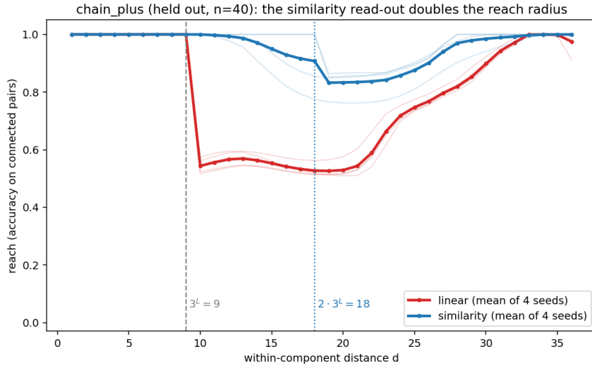
Figure 6: Table 22 drawn out (held-out chain_plus , mixed training, n = 40 ; thick = mean of four seeds, thin = per seed). Linear (red) drops right after 3^L = 9 ; similarity (blue) holds to \approx 2 \cdot 3^L = 18 . Both recover on the farthest pairs.
