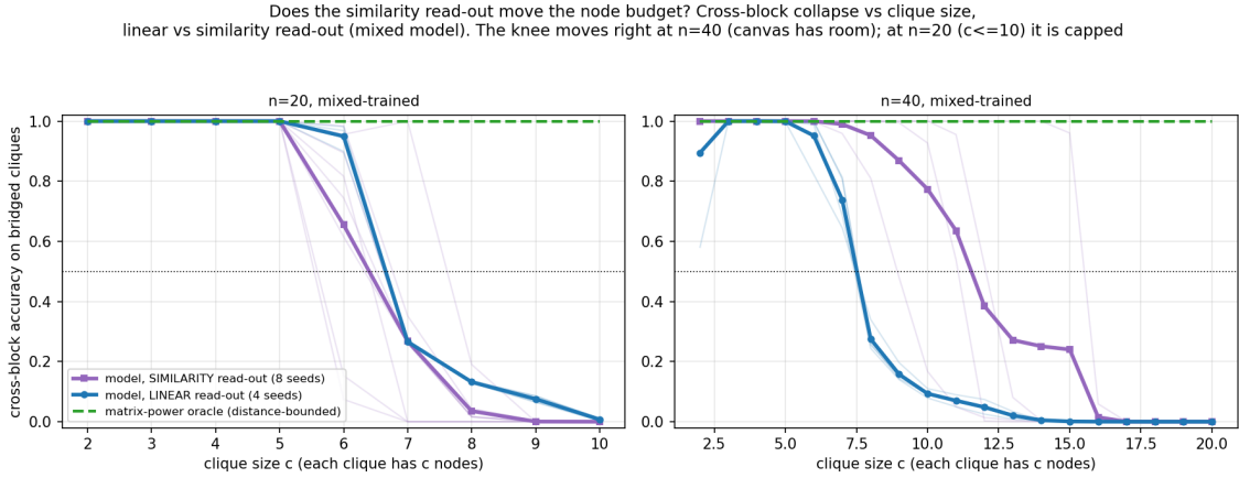
Figure 9: Model : the base connectivity transformer (RoBERTa trunk, L = 2 , single head, d_{\text{model}} = 512 , full matrix \hat{R} ), mixed -trained, with the linear (blue) vs the similarity (purple) read-out; eval-only , eight seeds at n = 20 / four at n = 40 for similarity, four for linear (thin = seeds, thick = mean). Test set : bridged cliques, \geq 400 graphs per clique size. Metric : cross-block pair accuracy vs clique size c ; the green dashed line is the matrix-power oracle (flat at 1, bridge \leq 3 hops). At n = 40 (right) the similarity read-out holds the bridge across a larger clique — the knee moves from c \approx 7 to c \approx 11 –12 — the same meet-in-the-middle that doubles the distance reach in Report IV. At n = 20 (left) the cliques fill the canvas by c = 10 , so the larger budget cannot be exercised and the knee is unchanged. Neither read-out connects the bridge at the full clique size: the wall is moved, not removed.
