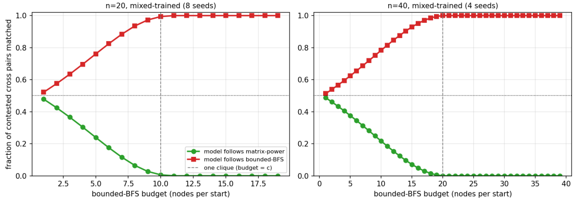
Figure 5: Model : the mixed -trained base connectivity transformer (RoBERTa trunk, linear read-out, L = 2 , single head, d_{\text{model}} = 512 , full-matrix \hat{R} ), eval-only, eight seeds at n = 20 / four at n = 40 ; n = 20 (left), n = 40 (right). Test set : bridged cliques at full clique size, 500 graphs. Metric : restricted to the cross pairs where the matrix-power oracle and the visit-bounded-BFS oracle disagree (the bridge pairs), the fraction the model matches to each oracle, as the BFS budget b varies. The model tracks the early-stopping BFS, not matrix powering: as b approaches one clique (dashed line) the model matches BFS on \rightarrow 1.0 of the contested pairs and matrix powering on \rightarrow 0 . This is the same fact as the cross collapse, read against the two reference algorithms.
