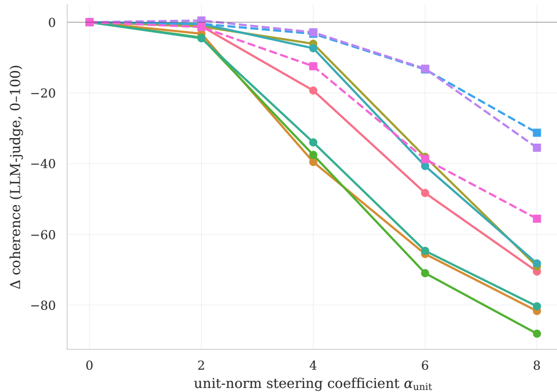
(b) Coherence cost dose-response @ L=17, unit-norm vectors
