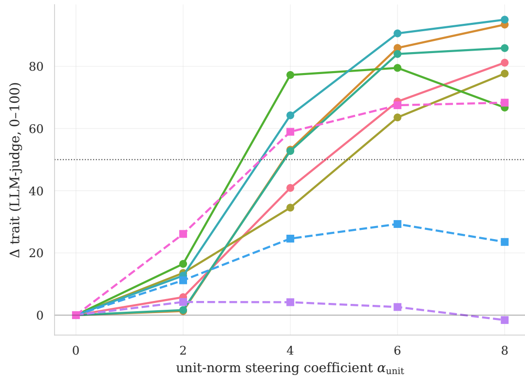
(a) Trait expression dose-response @ L=17, unit-norm vectors
