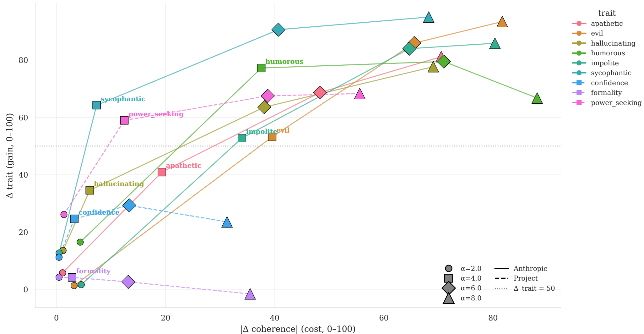
Trait gain vs coherence cost @ L=17, unit-norm — \alpha_{\text{unit}} \in \{2,4,6,8\}
