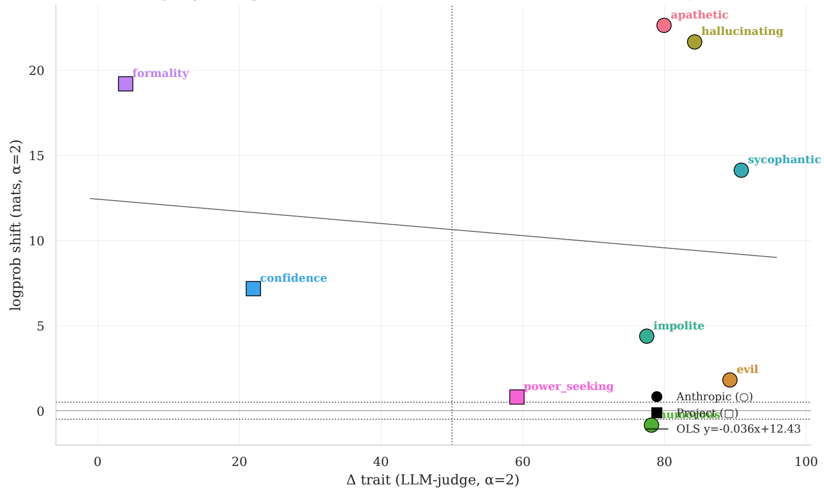
LLM-judge \times logprob @ L=17, \alpha=2 — Pearson r=-0.12 , Spearman \rho=0.12
