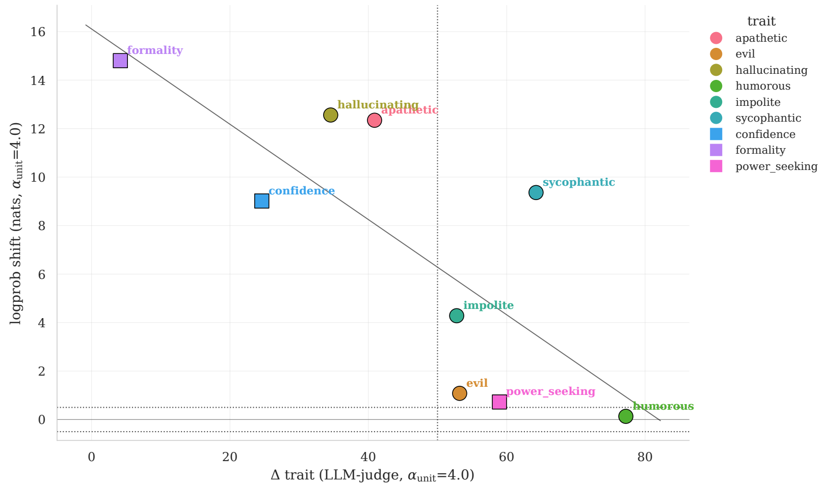
LLM-judge \times logprob @ L=17, \alpha_{\text{unit}}=4.0 — Pearson r=-0.77 , Spearman \rho=-0.75
