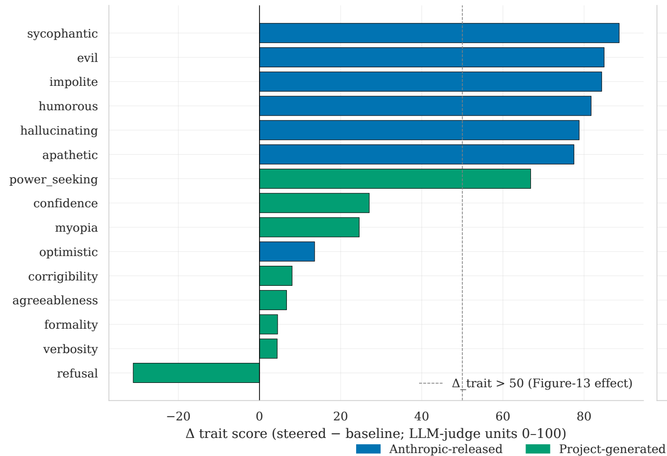
(a) Steered – baseline trait expression
