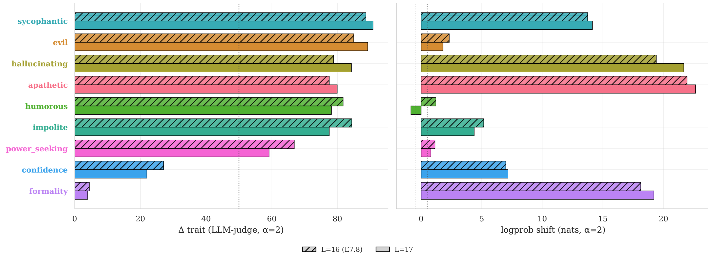
(a) LLM-judge
