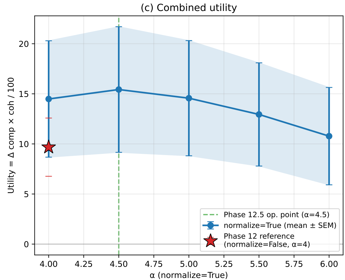
Phase 15 pilot — aggregate dose-response under normalize=True mean across 5 pairs (apathetic+power_seeking excluded — broken trait); green dashed line = Phase 12.5 committed operating point ( \alpha = 4.5 )
