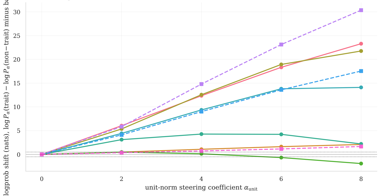
Logprob shift dose-response @ L=17, unit-norm vectors (MWE test split)
