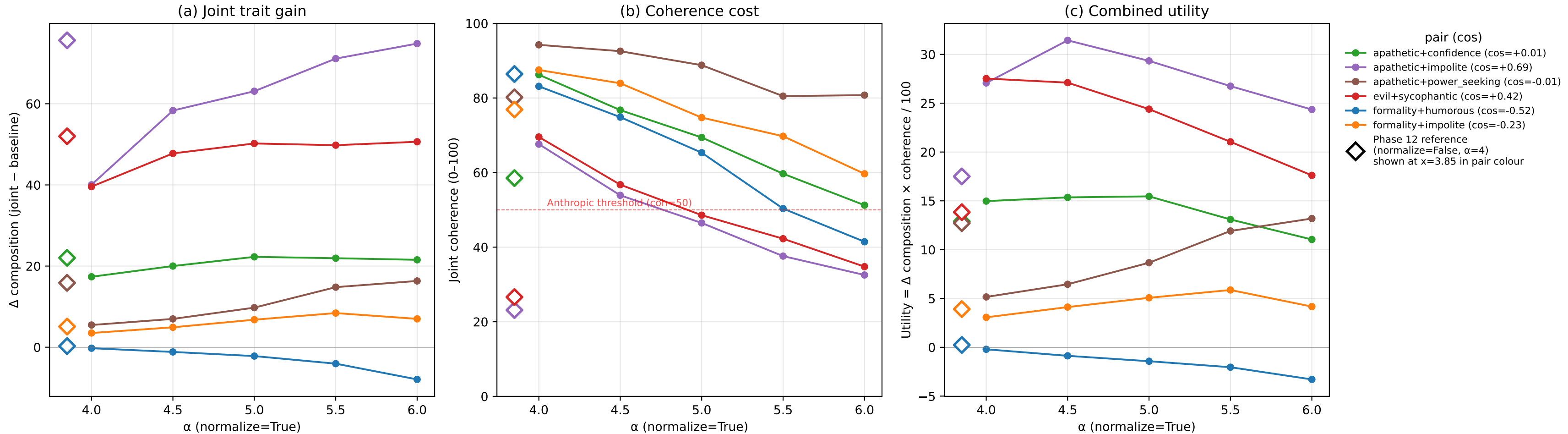
Phase 15 pilot — per-pair dose-response under normalize=True
