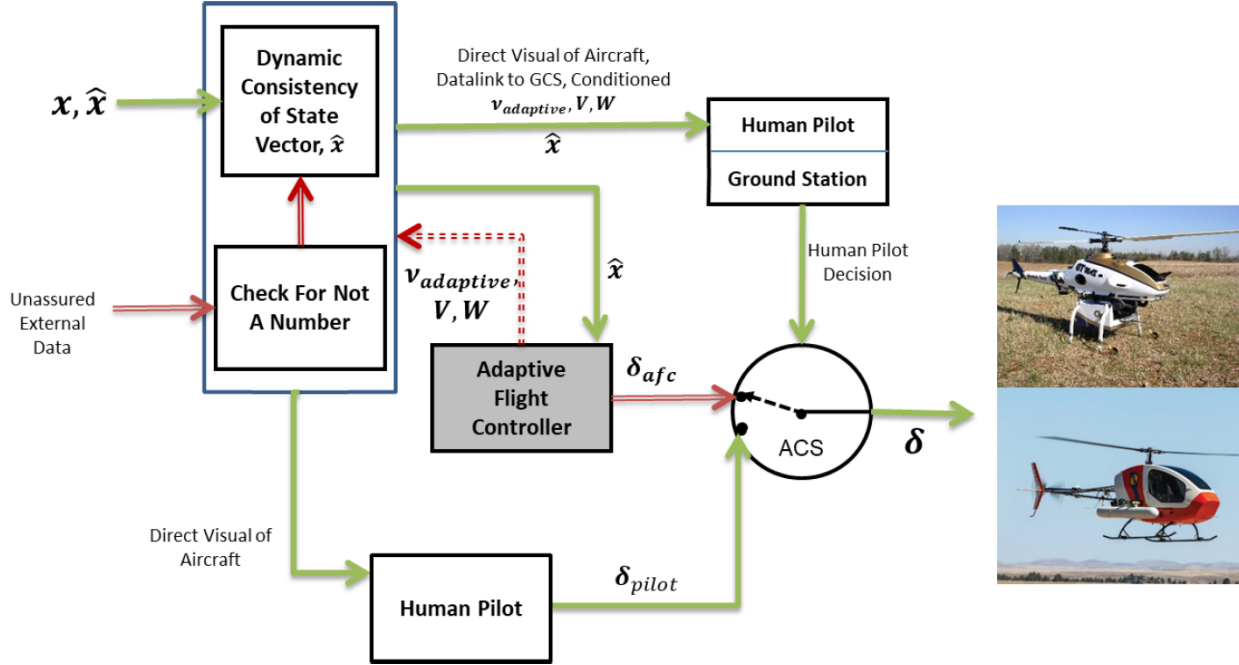
Figure 7 RTA system for an adaptive controller with human-in-the-loop
