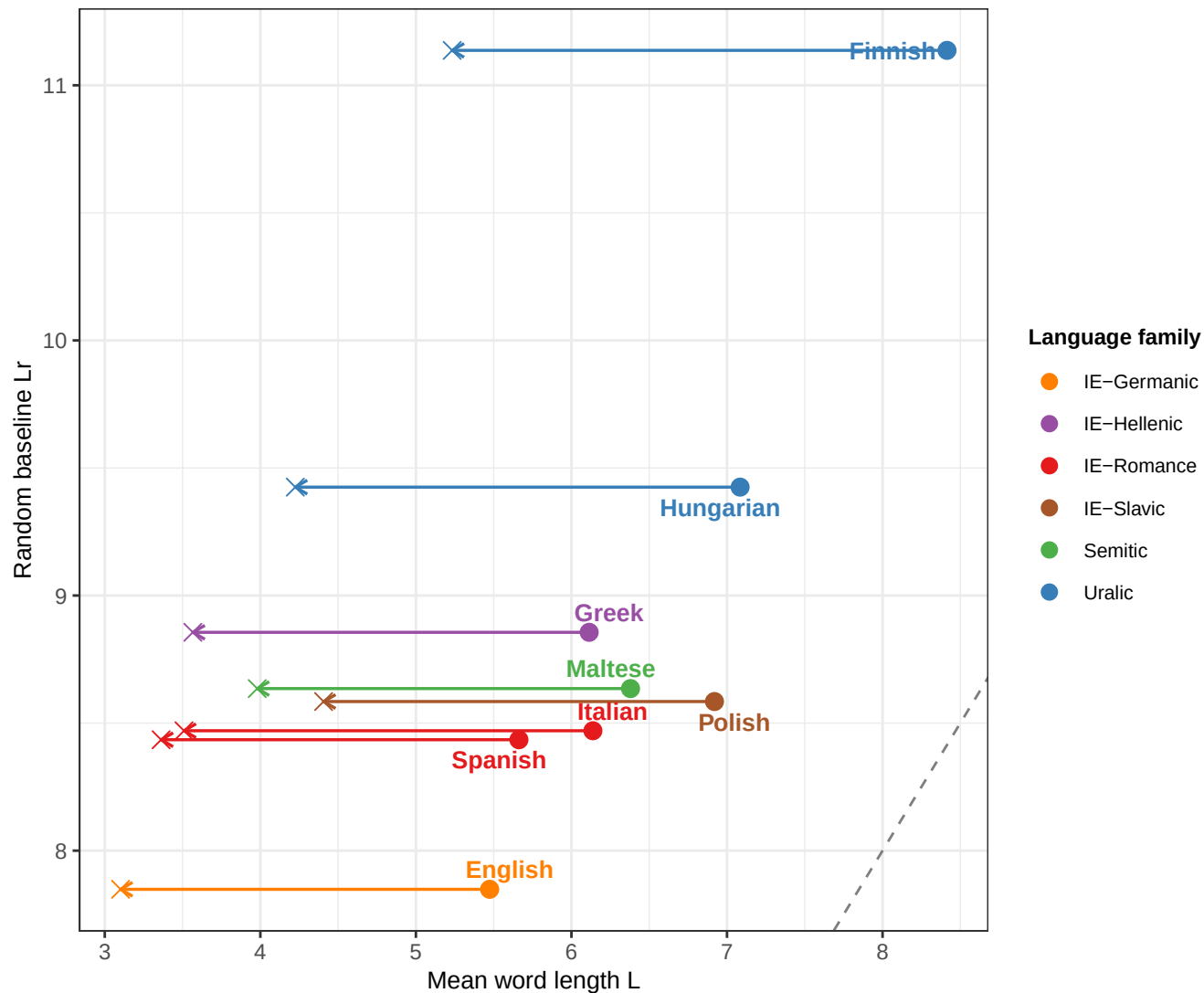
Degree of compression across languages
