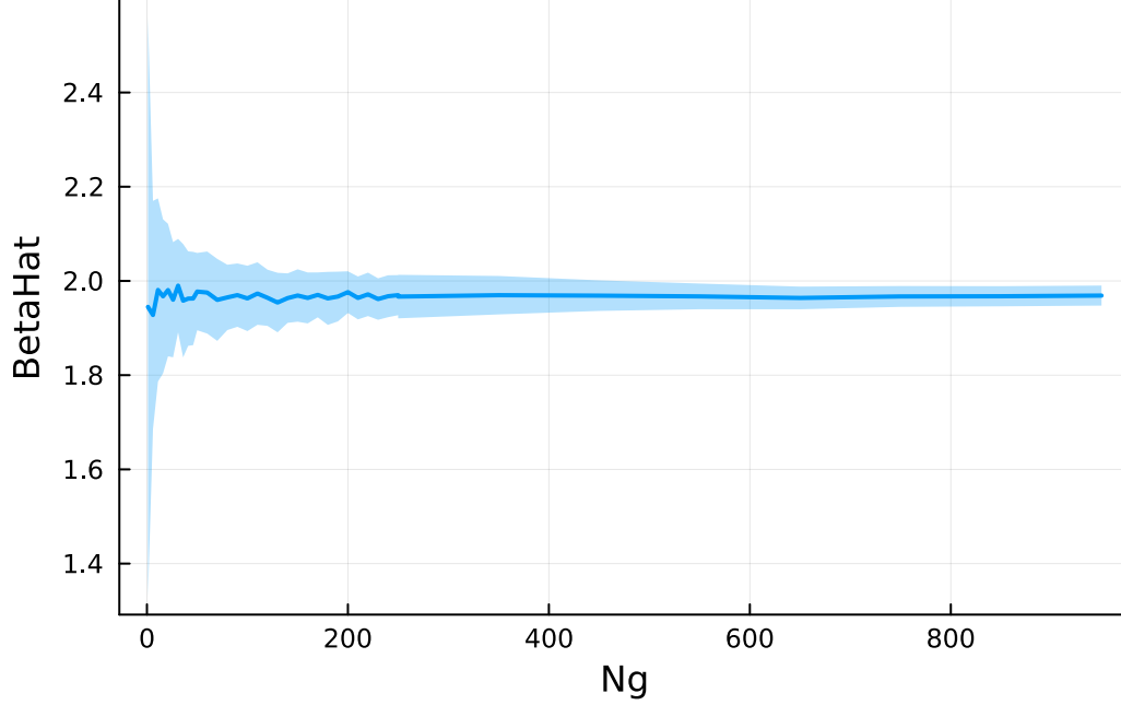
Figure 3: Consistency of betahat as N_g
