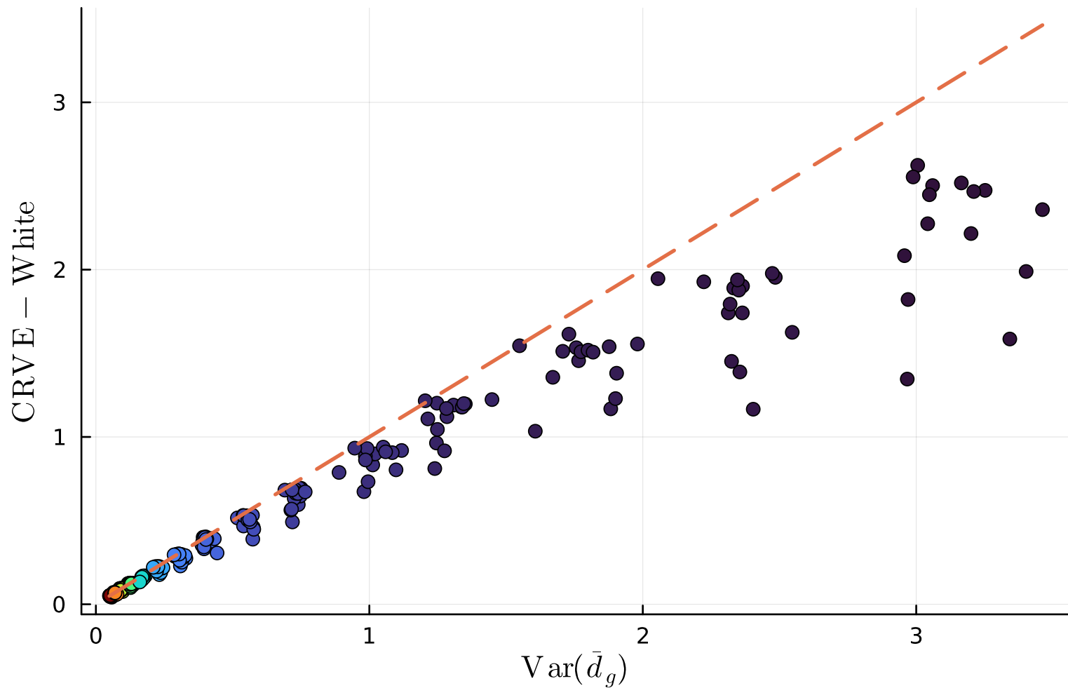
CRVE – White vs \text{Var}(\text{mean}(\bar{d}_g))
