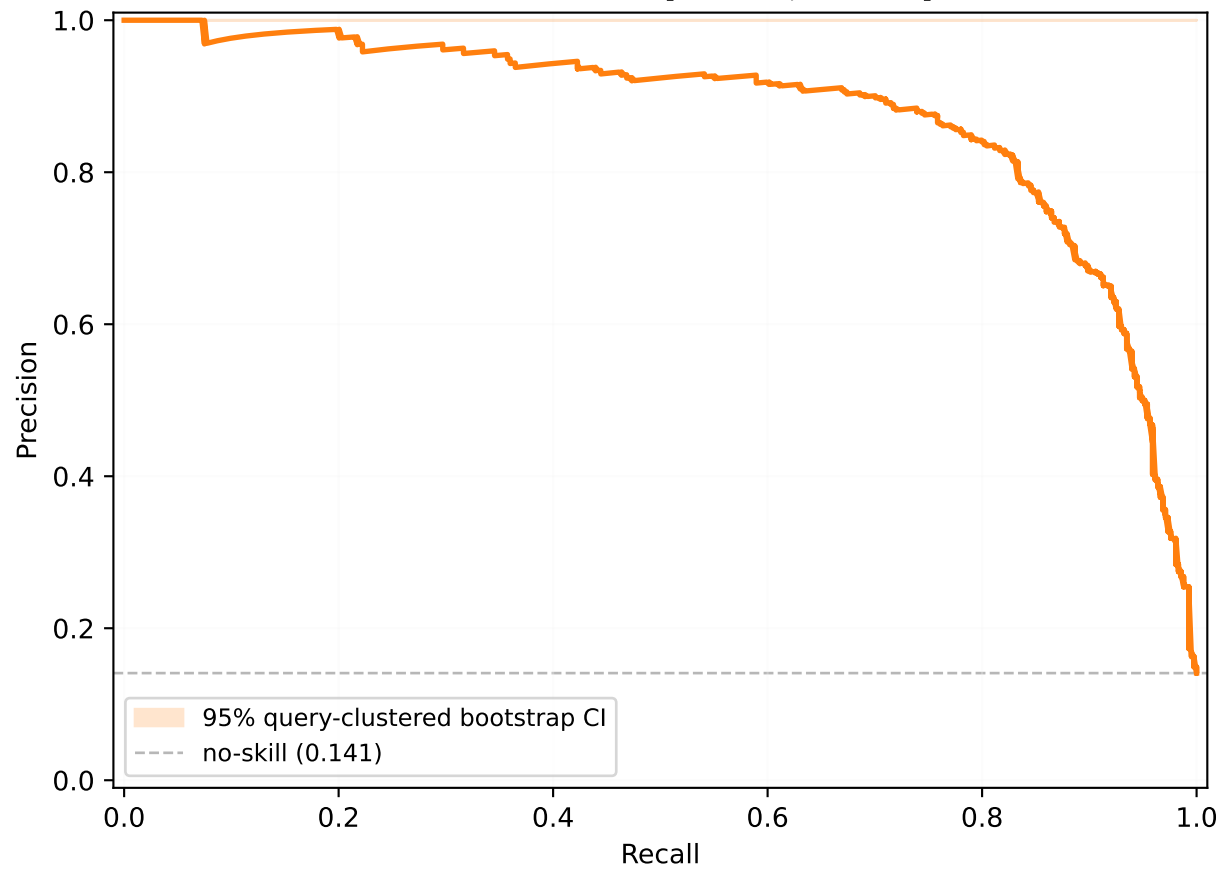
(b) Precision-Recall curve AUPRC = 0.8771 [0.8477, 0.9042]
