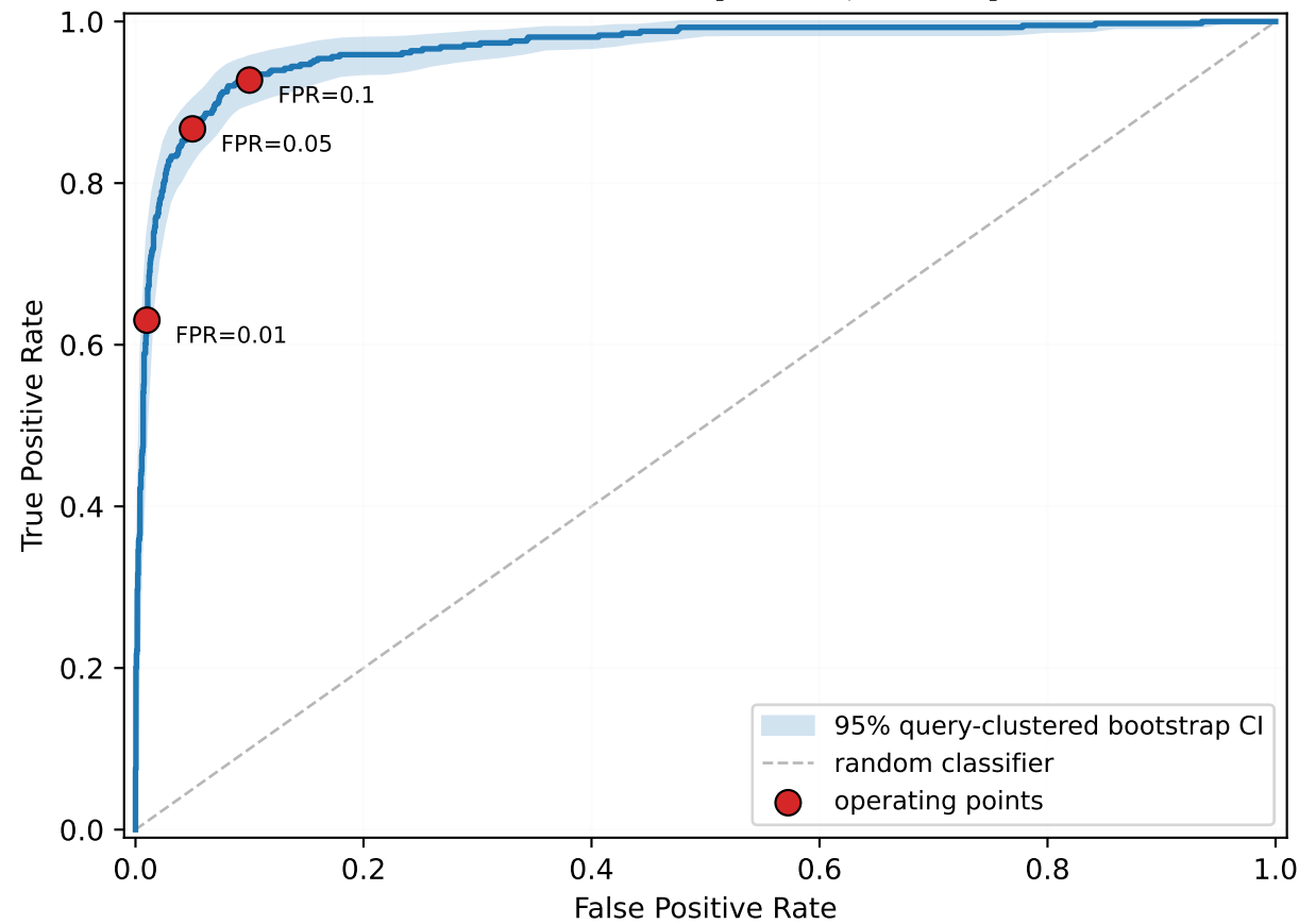
(a) ROC curve AUROC = 0.9666 [0.9554, 0.9767]
