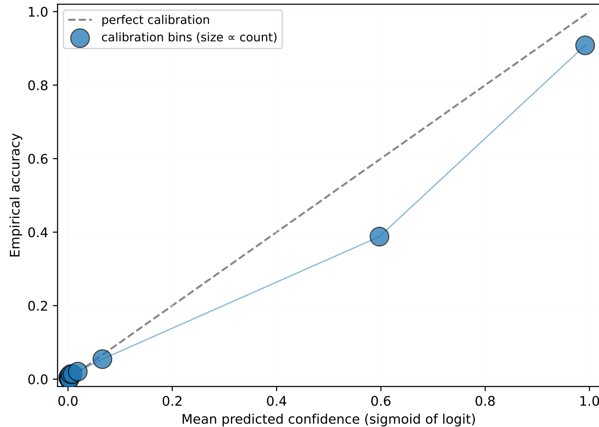
(a) Reliability diagram (10 quantile bins)
