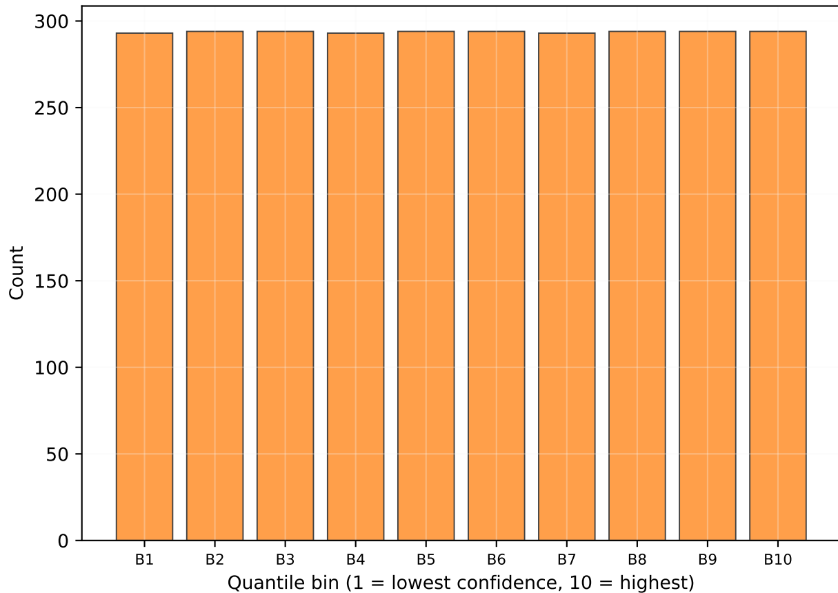
(b) Bin counts (quantile binning, equal sample size)
