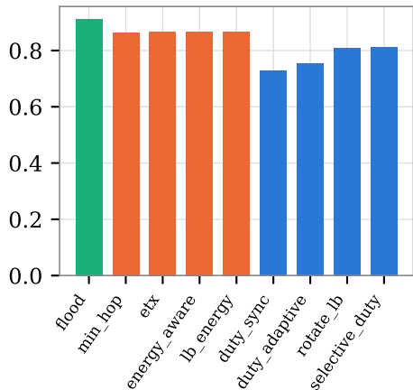
Packet delivery ratio
