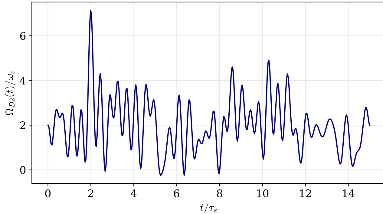
CRAB — Qubit 2 (F=0.9935)
