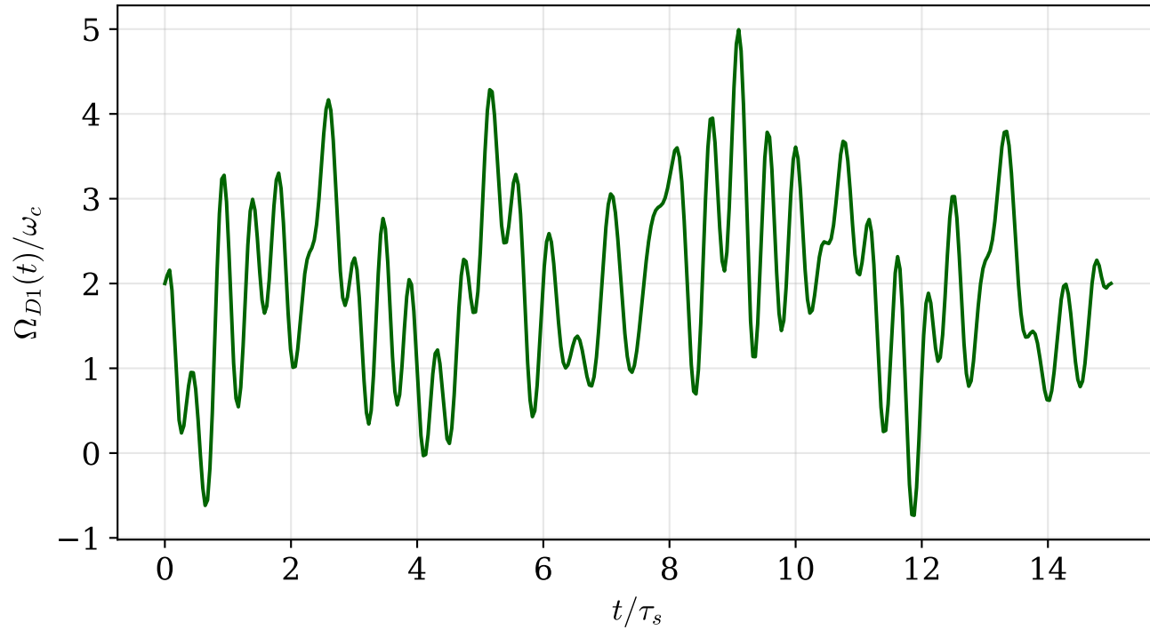
CRAB — Qubit 1 (F=0.9935)
