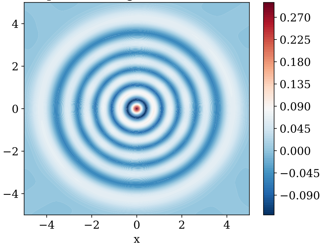
Optimized Wigner ( F=0.9877 )
