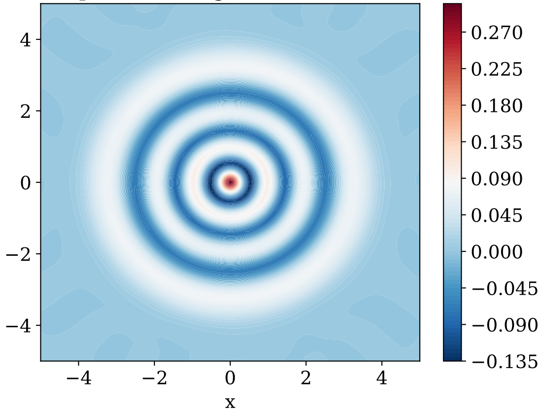
Optimized Wigner ( F=0.9908 )
