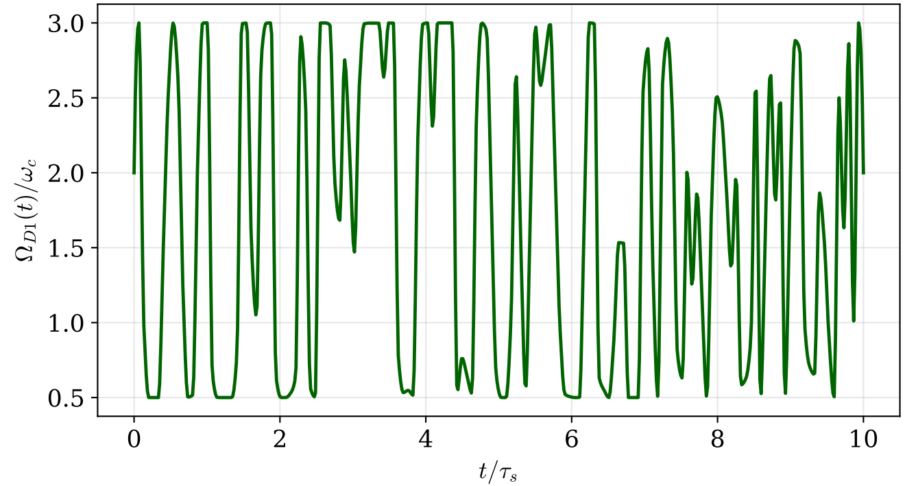
Smoothed PCHIP — Qubit 1 (F=0.9622)
