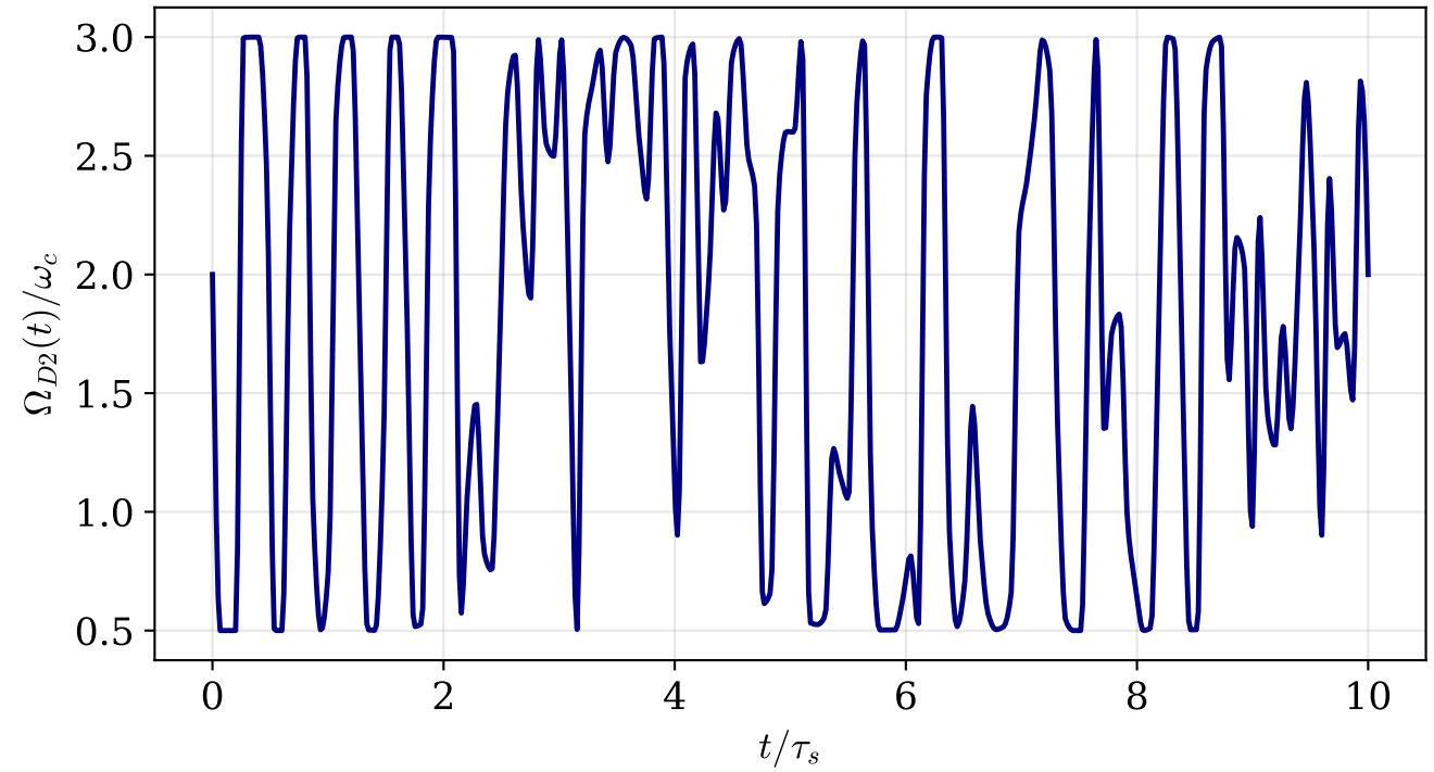
Smoothed PCHIP — Qubit 2 (F=0.9622)
