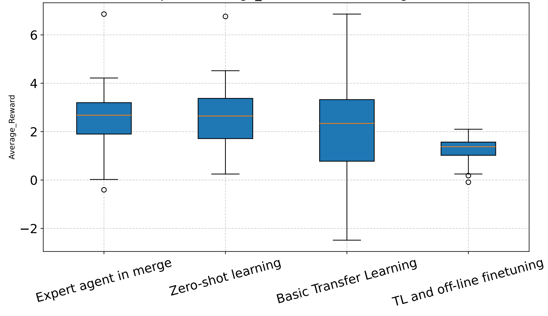
Boxplot of Average_Reward for Different Agents
