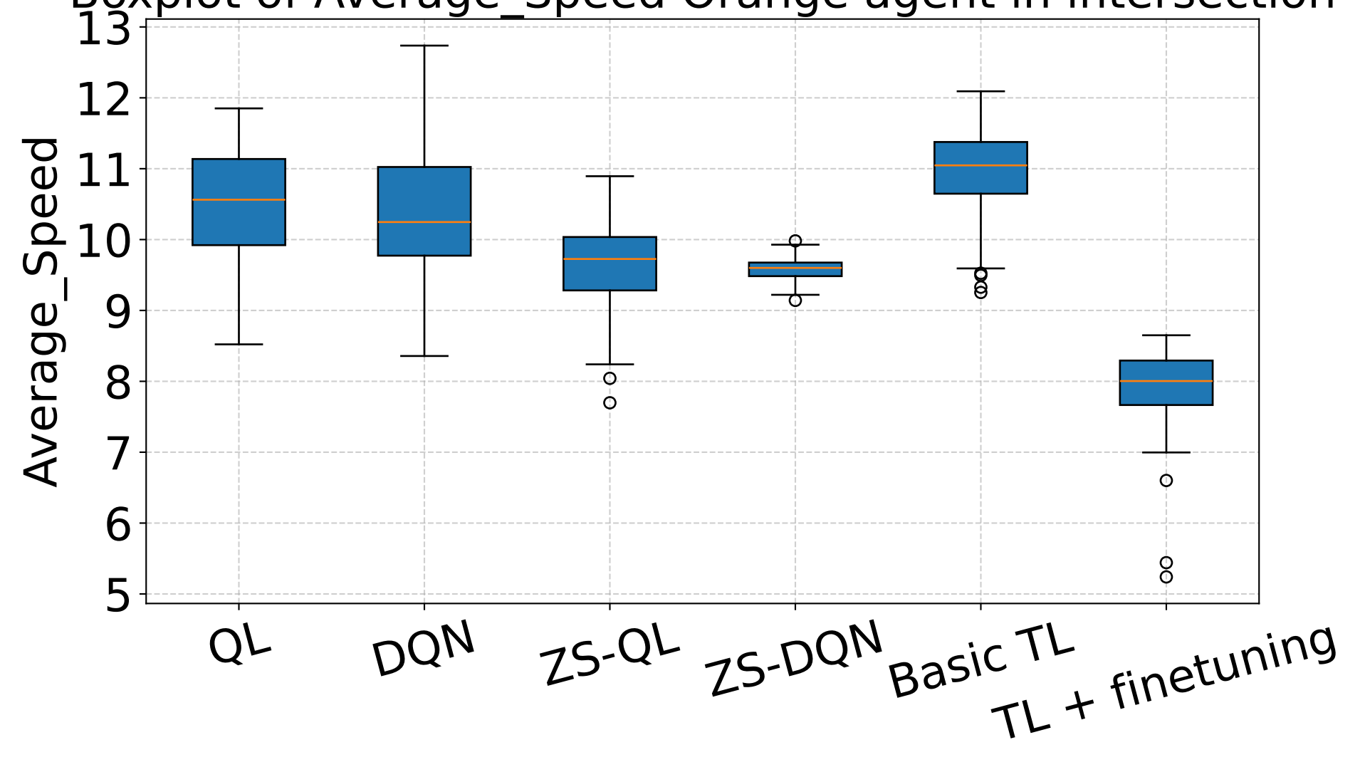
Boxplot of Average_Speed Orange agent in intersection
