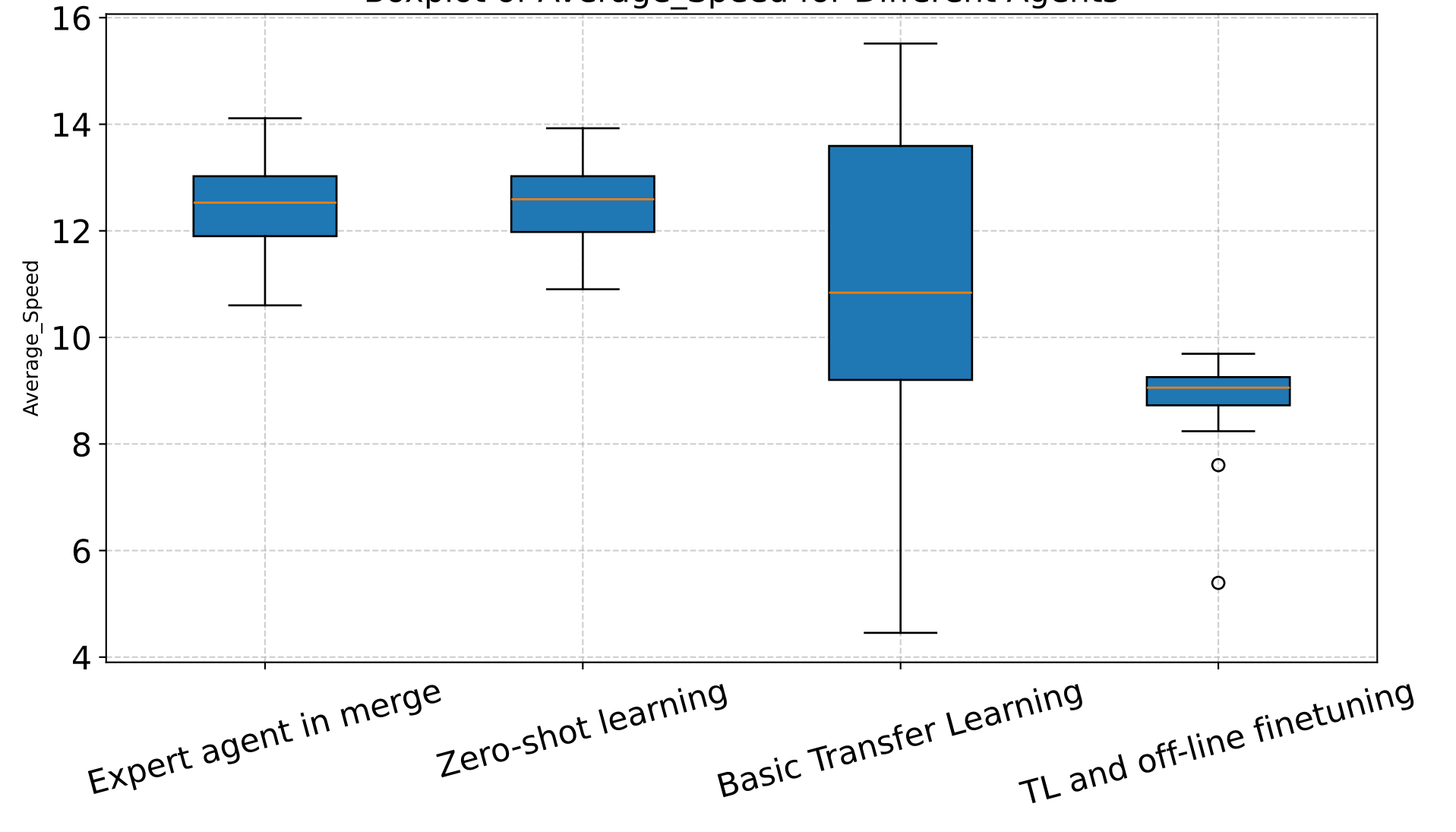
Boxplot of Average_Speed for Different Agents
