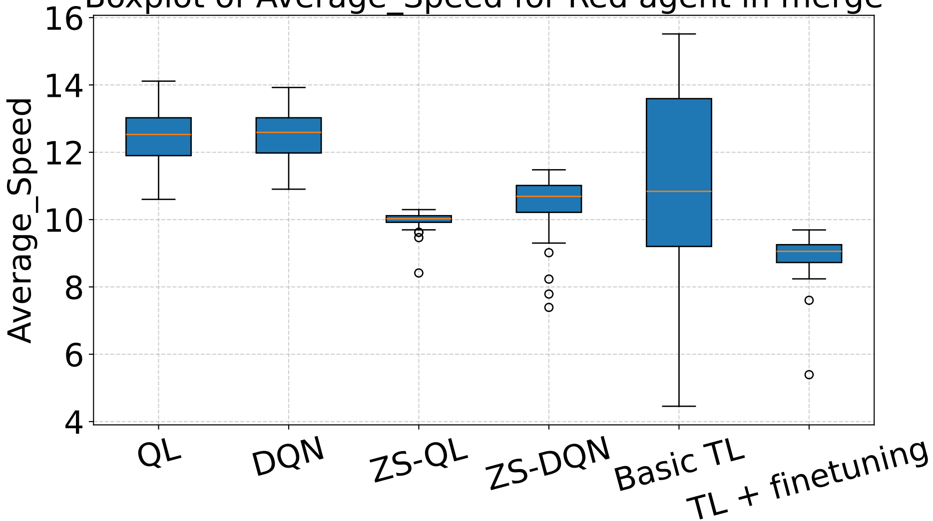
Boxplot of Average_Speed for Red agent in merge
