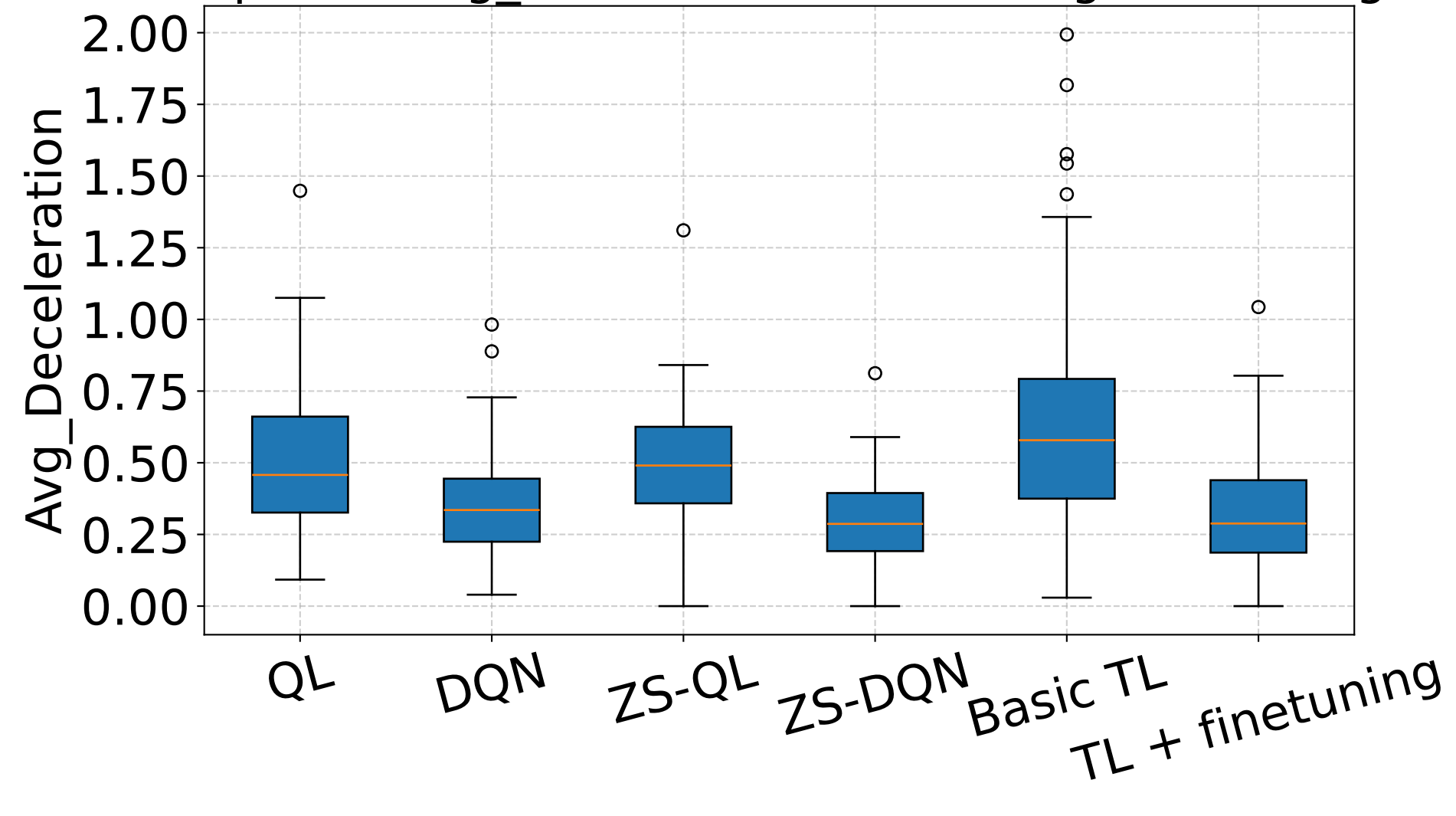
Boxplot of Avg_Deceleration for Red agent in merge
