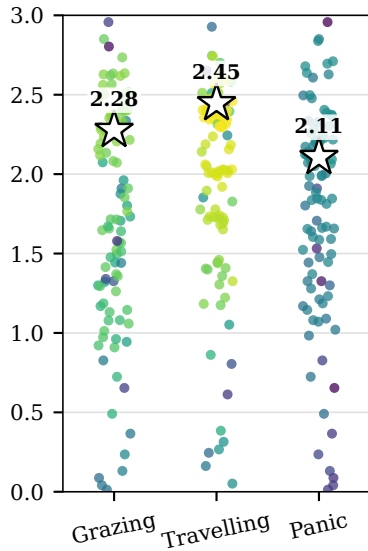
Cognitive coefficient c_1
