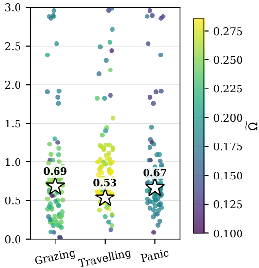
Social coefficient c_2
