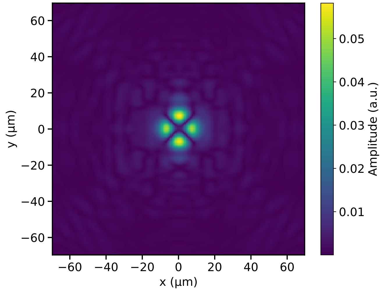
Projected Amplitude
