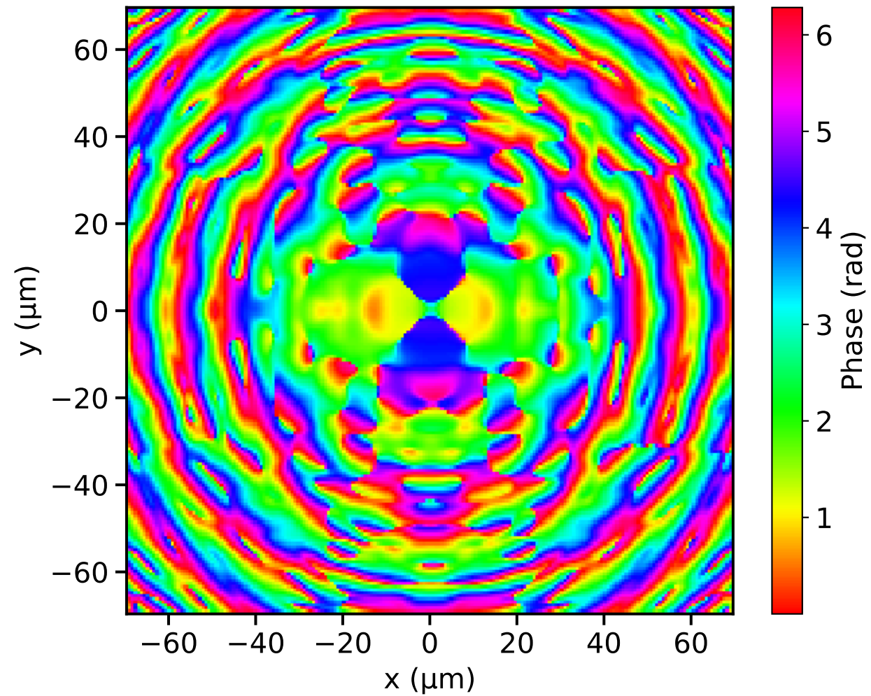
Projected Phase
