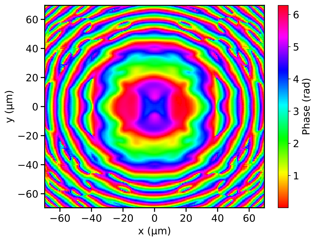
ASM - Intermediate Field Phase
