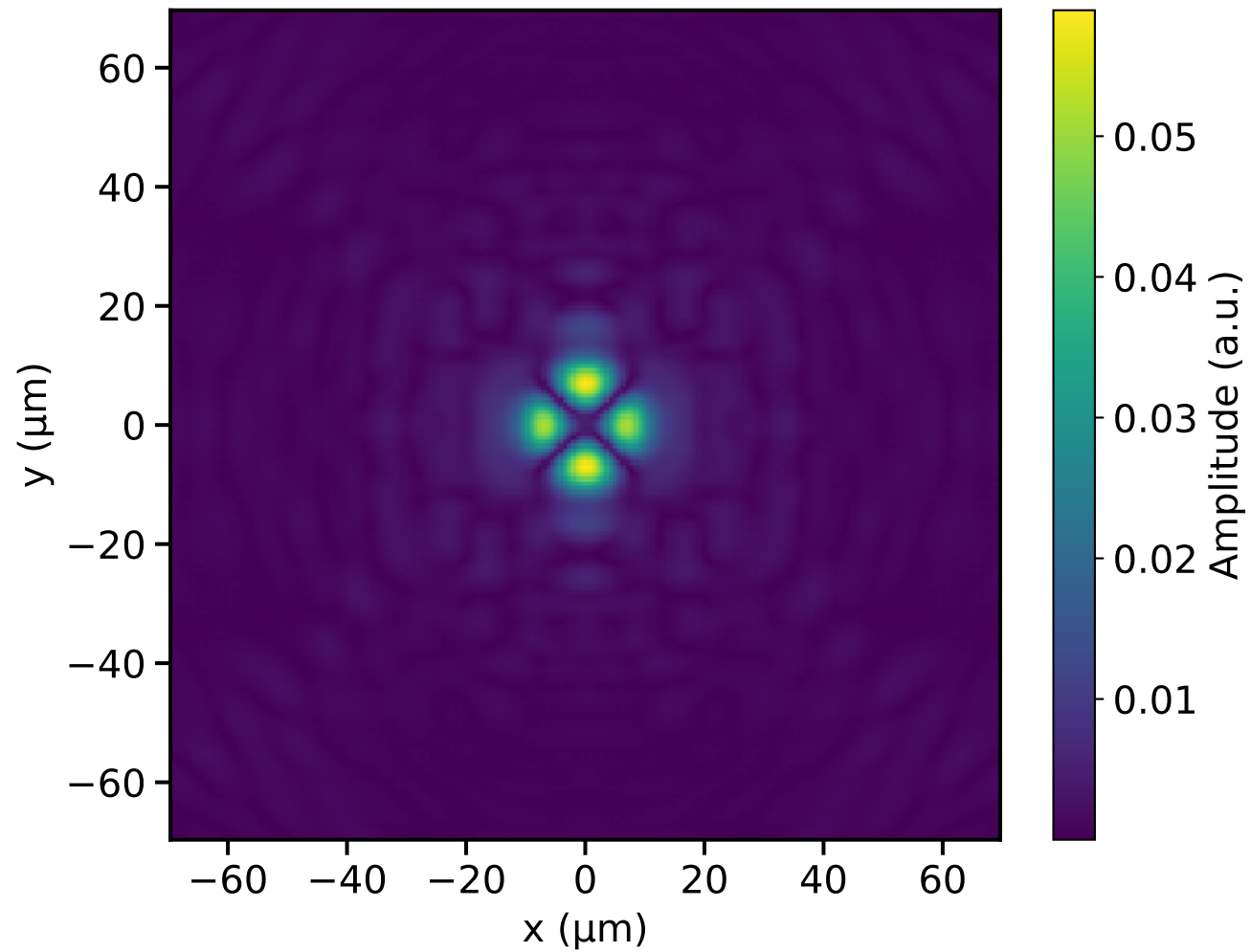
ASM Output Field Amplitude
