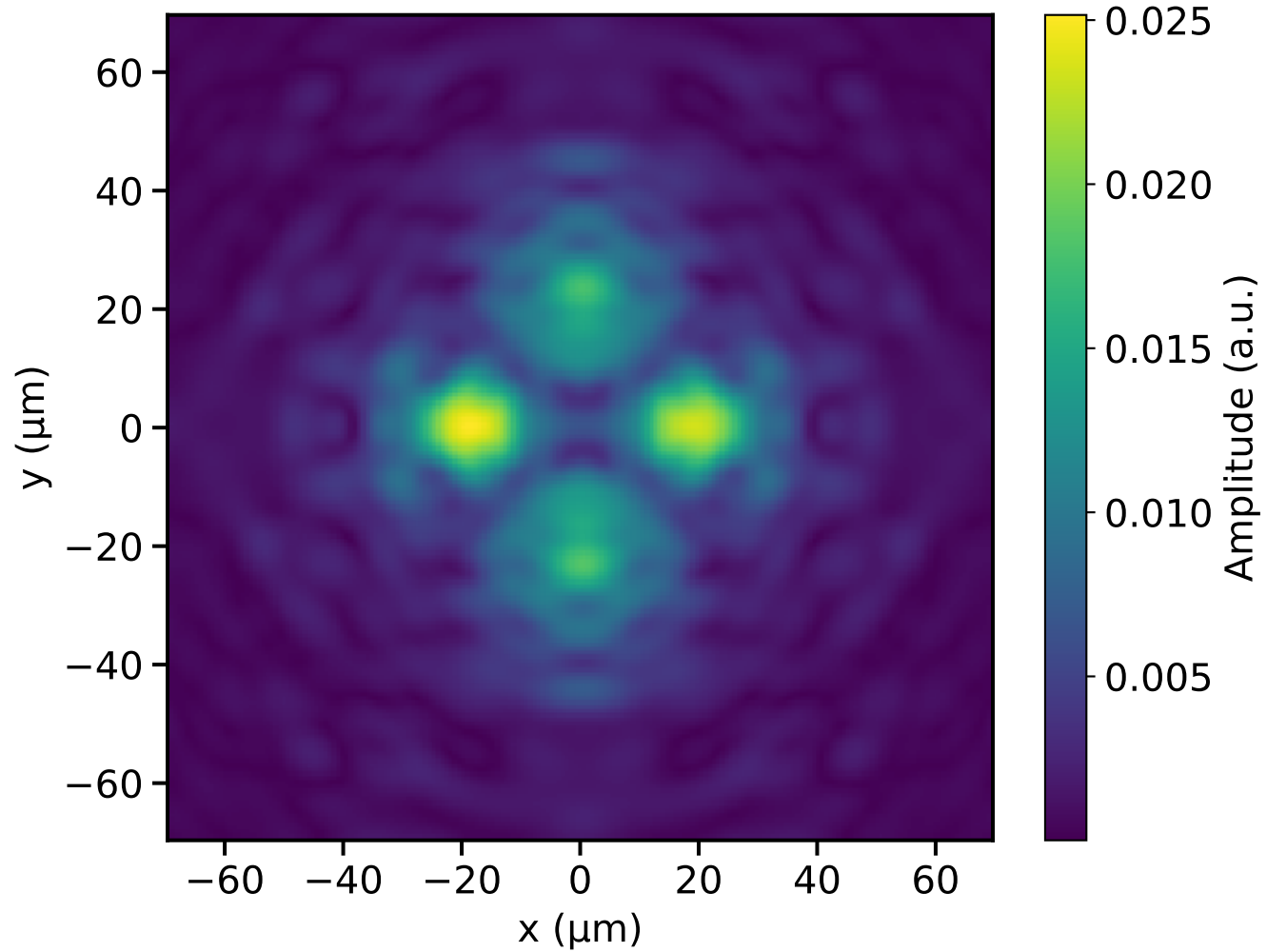
FDTD - Projected Amplitude
