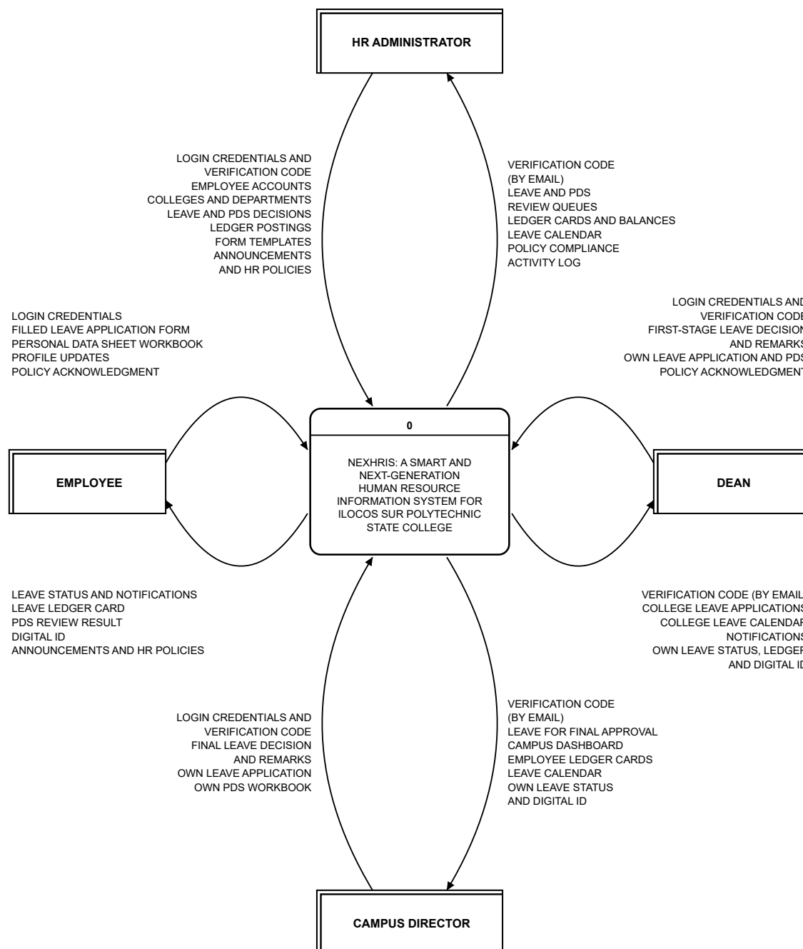
CONTEXT DIAGRAM (LEVEL 0) OF NEXHRIS: A SMART AND NEXT-GENERATION HUMAN RESOURCE INFORMATION SYSTEM FOR ILOCOS SUR POLYTECHNIC STATE COLLEGE
