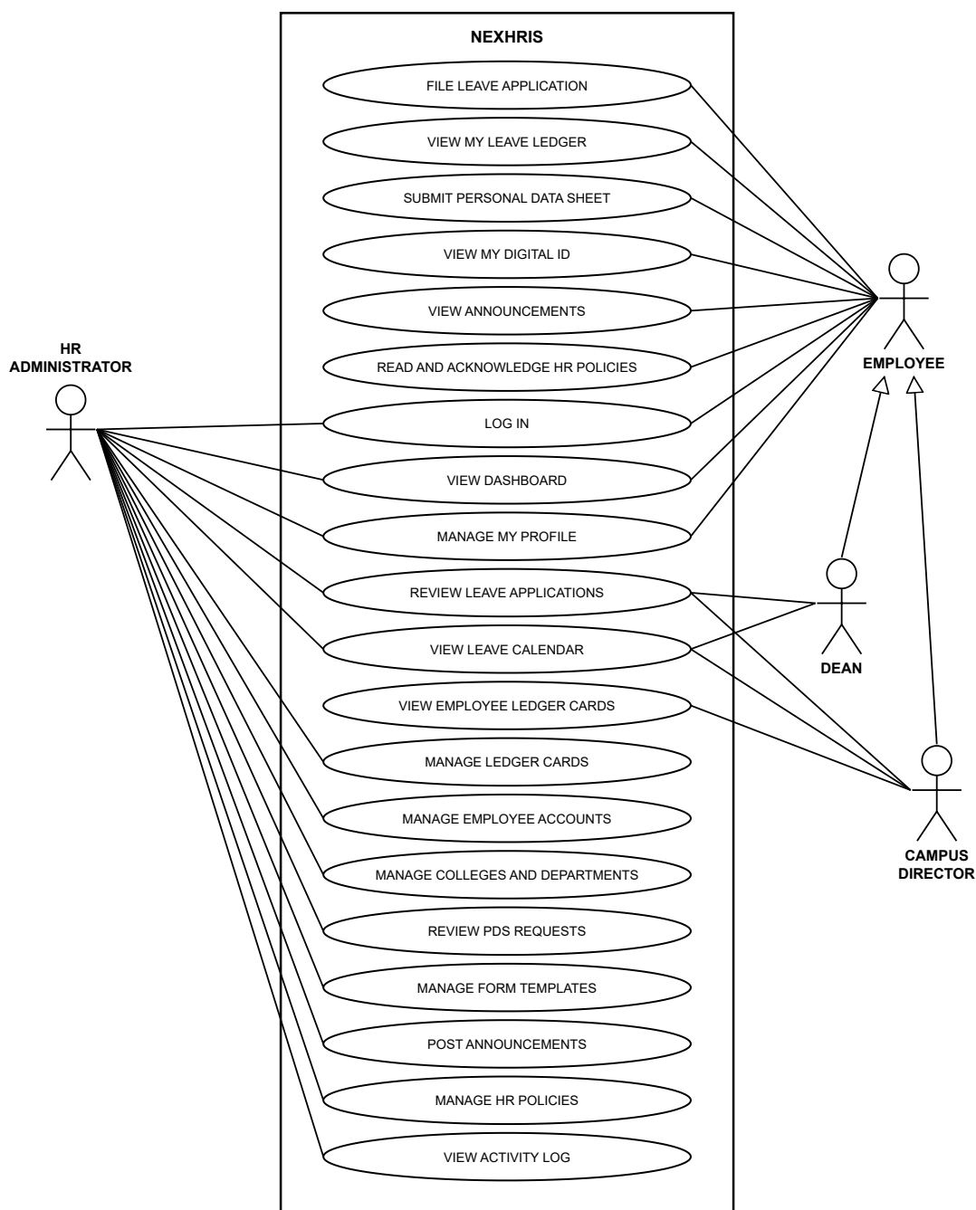
USE CASE DIAGRAM OF NEXHRIS: A SMART AND NEXT-GENERATION HUMAN RESOURCE INFORMATION SYSTEM FOR ILOCOS SUR POLYTECHNIC STATE COLLEGE
