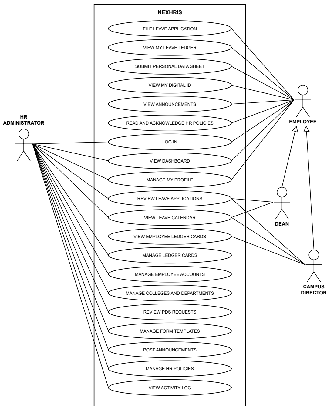
USE CASE DIAGRAM OF NEXHRIS: HUMAN RESOURCE INFORMATION SYSTEM FOR ISPSC TAGUDIN CAMPUS
